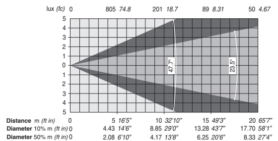
Maximum Zoom with ovalizer filter (Y axis)
