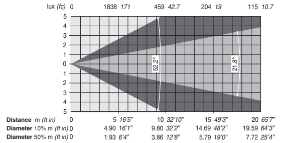
Maximum Zoom (52.2° 10% - 21.8° 50%)
