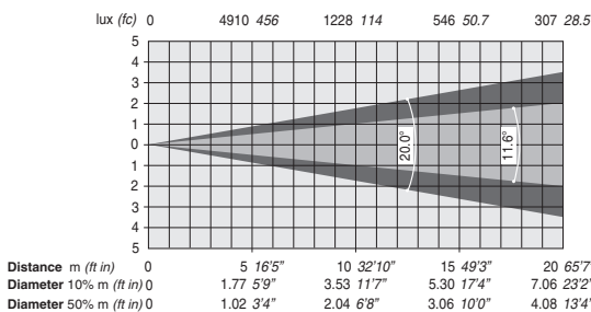
Minimum Zoom with ovalizer filter (Y axis)
