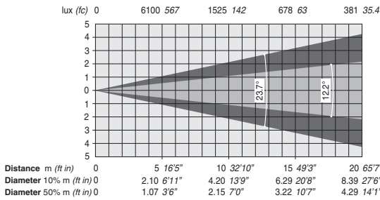
Minimum Zoom with 100% Frost (23.7° 10% - 12.2° 50%)
