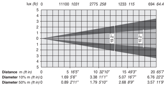
Minimum Zoom (19.2° 10% - 10.2° 50%)
