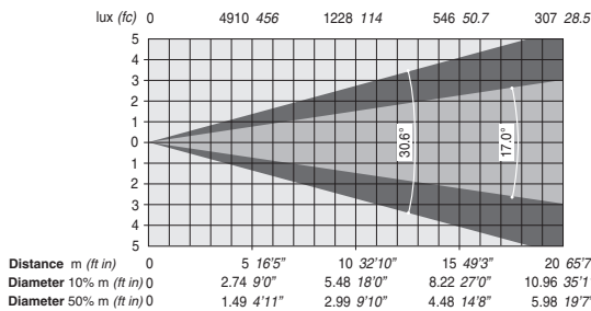
Minimum Zoom with ovalizer filter (X axis)
