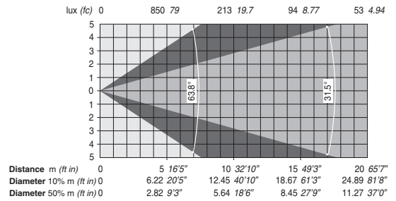
Maximum Zoom with 100% Frost (63.8° 10% - 31.5° 50%)
