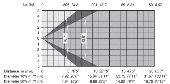
Maximum Zoom with ovalizer filter (X axis)
